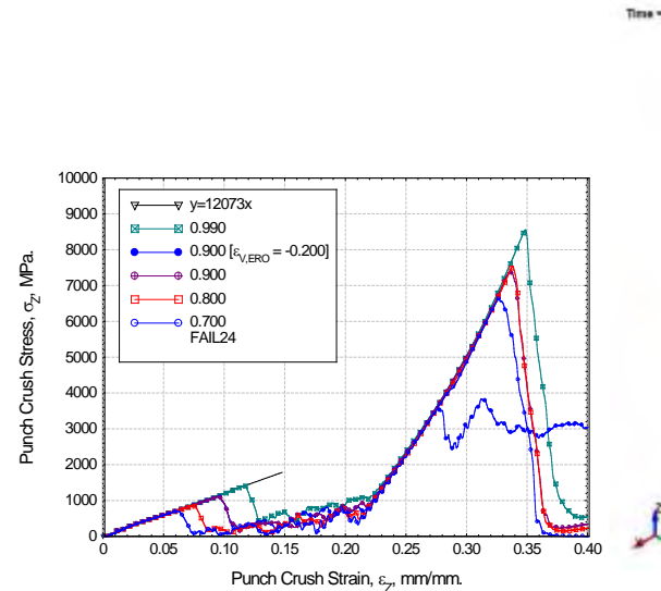
Prediction of Punch Crush Strength = 1400 MPa
