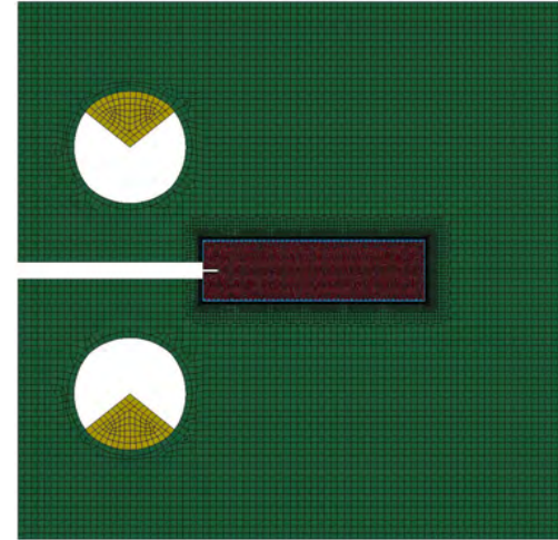
Compact Tension Microscale Fracture Model
