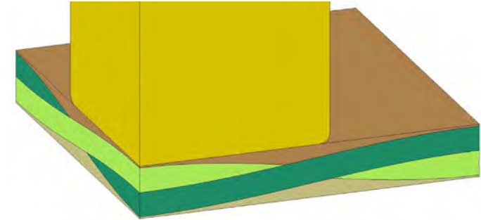
V_I = 200 m/s Impact Local Tow-tow Delamination and Cone Wave Initiation
